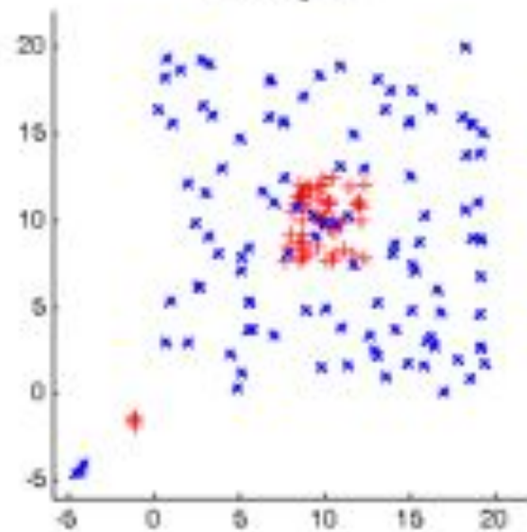
Training Set
